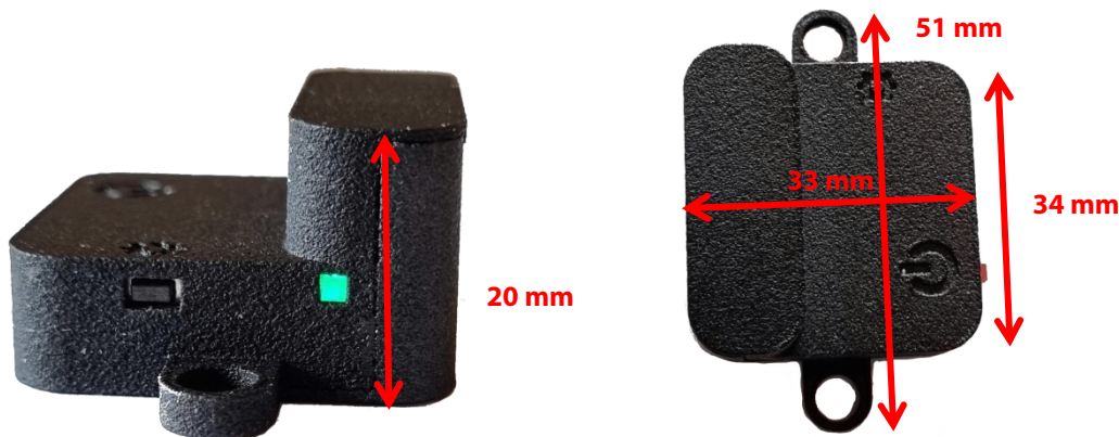
Figure 1 - DroneBeacon 150-serie transponder
